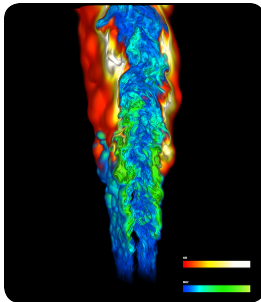
Direct numerical simulation reveals turbulent combustion of a lifted ethylene/air jet flame in a heated coflow of air. Computation by Chun Sang Yoo and Jackie Chen of Sandia National Laboratories. (Rendering courtesy of Hongfeng Yu, Sandia National Laboratories)
